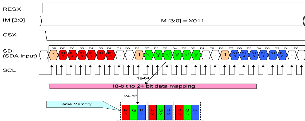
Figure 129: SPI Data for 18-bit/pixel (RGB 6-6-6 bits input), 262K-color
