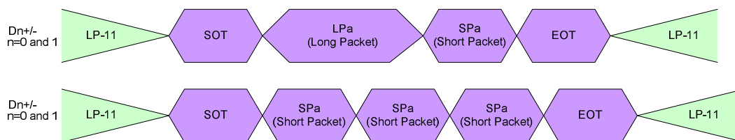
Figure 45: Multiple Packets in High-Speed Data Transmission – Examples
