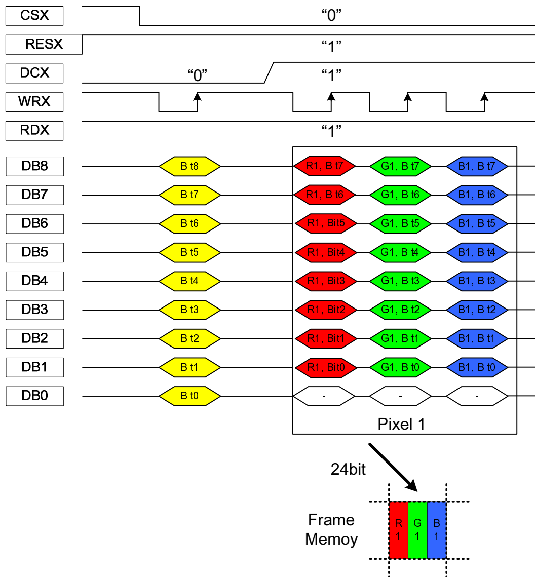
Figure 139: 9-bit Data Bus for 24-bit/pixel (RGB 8-8-8 bits input), 16.7M-color
