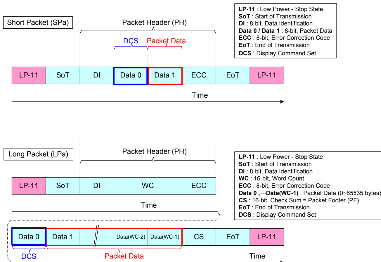
Figure 79: Display Command Set (DCS) in Short Packet (SPa) and Long Packet (LPa)
