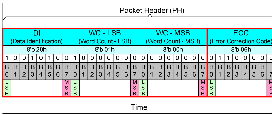
Figure 70: D [23...0] and P [7...0] of a Long Packet (LPa)
