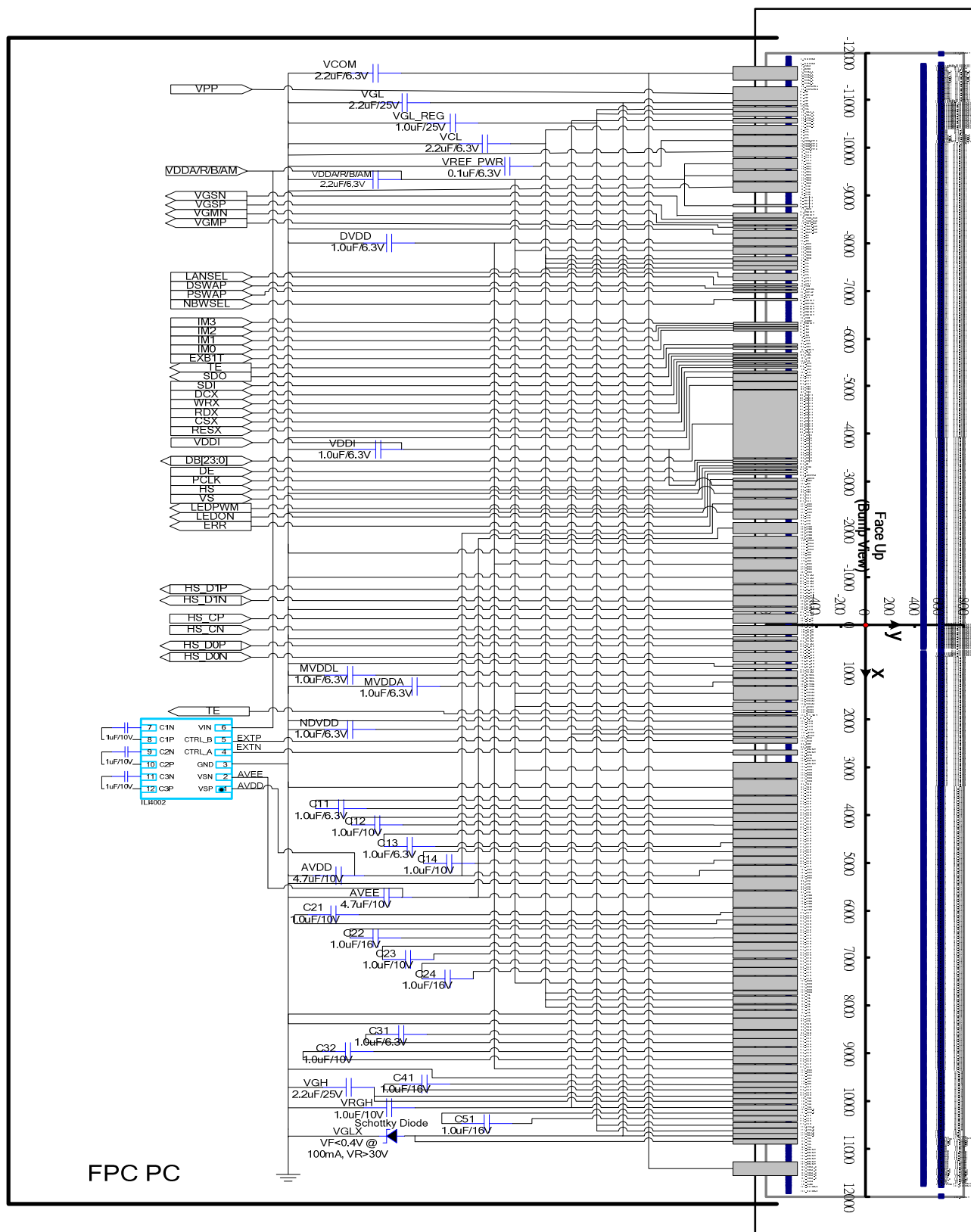
Figure 199: Reference Circuit
