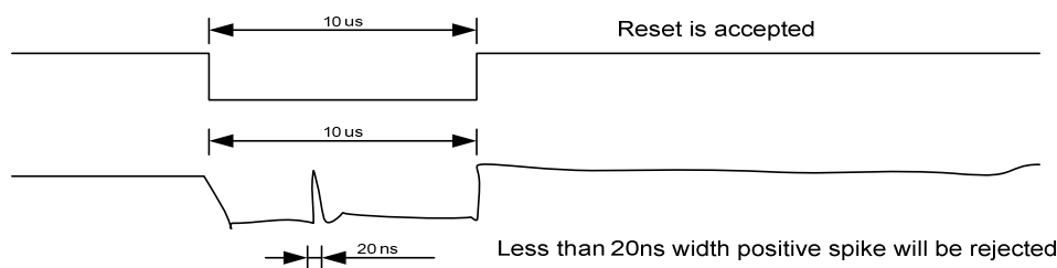
Figure 181: Positive Noise Pulse during Reset Low
