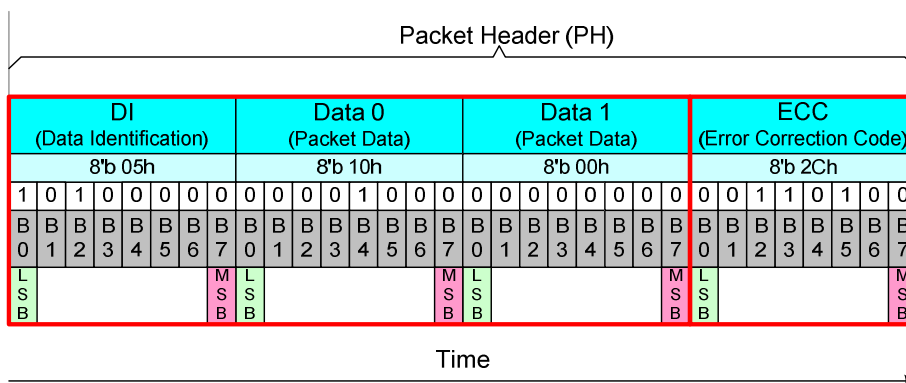
Figure 69: D [23...0] and P [7...0] of a Short Packet (SPa)
