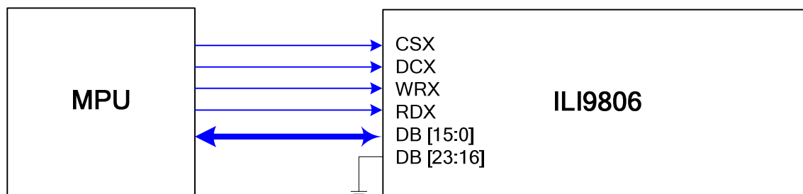
Figure 140: 16-bit Parallel MPU Interface
